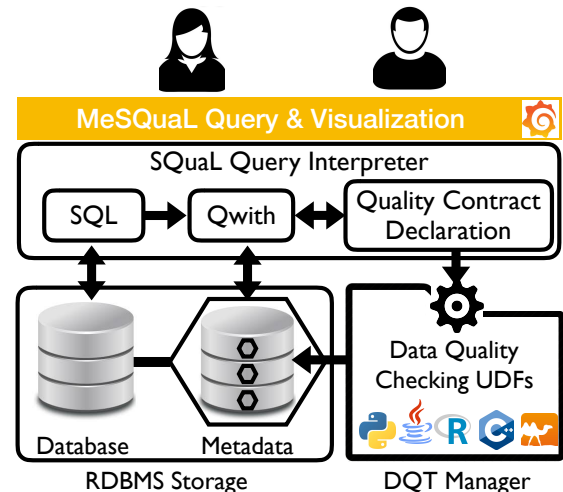
Figure 1: MeSQual Architecture.
